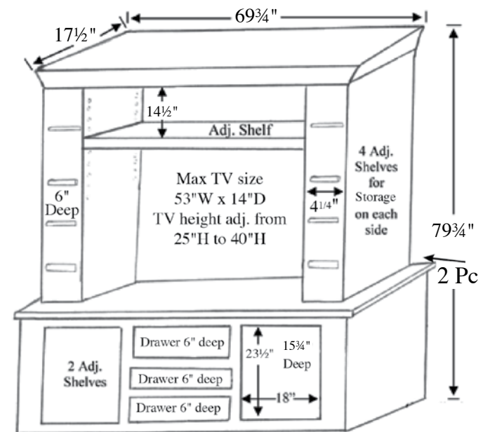
FVE-047-VS Base only: 67¼" W x 17¼" D x 30" H
